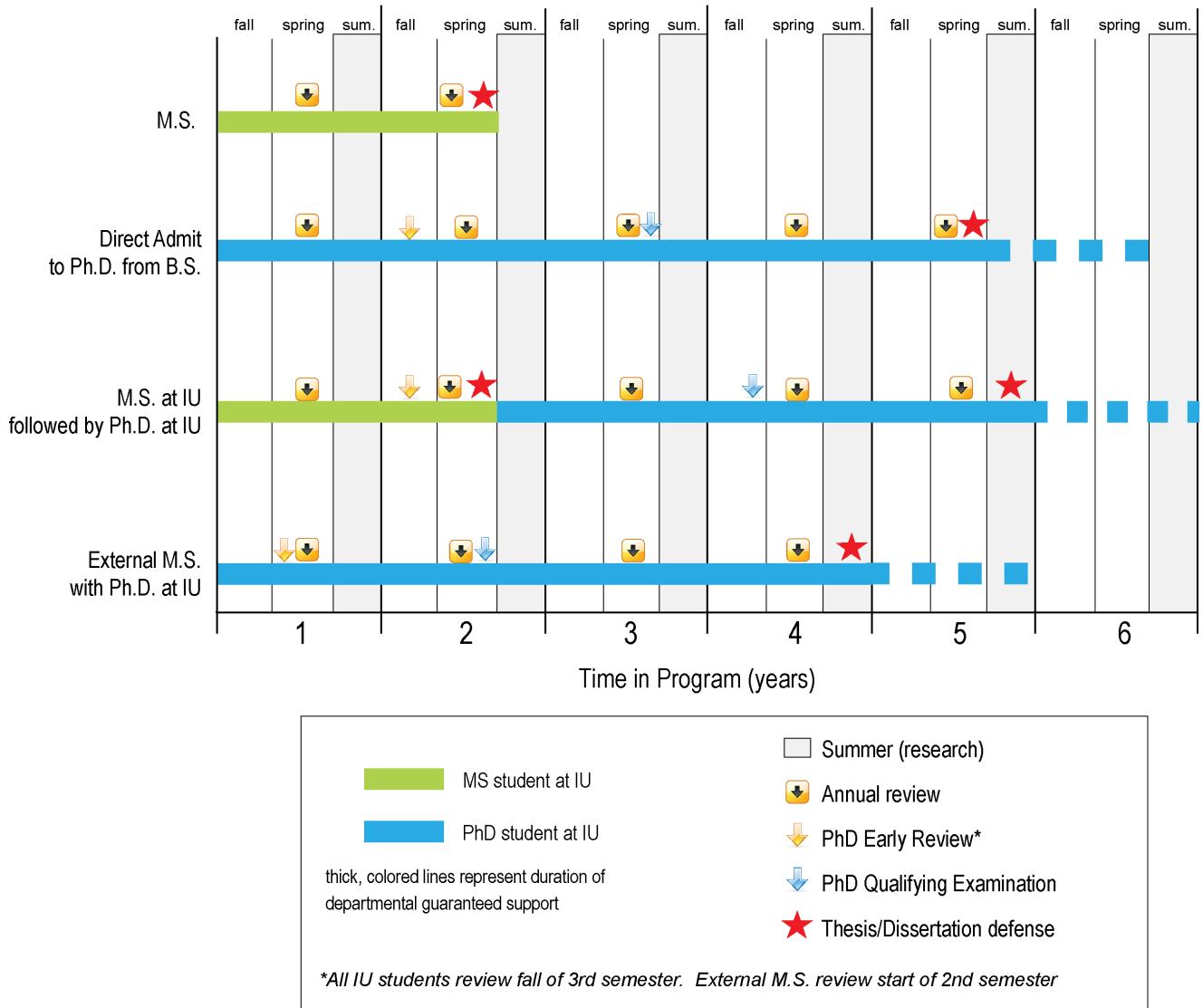
Figure 1: Illustrates a timeline for completing Ph.D. and M.S. degrees in Geological Sciences at IU.
